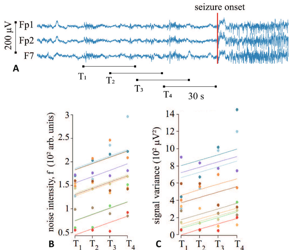
Fig. 11 A EEG data with seizure onset and four time intervals T_1 , T_2 , T_3 , T_4 that gradually approach the onset. Regression plots for noise intensity ( B ) and signal variance ( C ) in four time intervals T_1 , T_2 , T_3 , T_4 . Different colours correspond to data from different subjects. The lines have a similar slope: r = 0.52 for noise intensity and r = 0.38 for signal variance. Based on materials from Karpov et al. [86]
