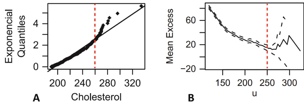
Fig. 1 Examples of exponential QQ plot for data exceeding the reference value of 190 mg/dL ( A ) and estimated mean excess function for the same data ( B ). The red dashed line marks the threshold. Based on materials from de Zea Bermudez and Mendes [38]
