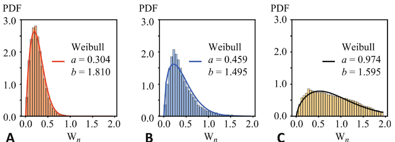
Fig. 9 PDFs of wavelet energy at 7 Hz (histograms) and fitted Weibull distributions (curves) with parameters a and b for different segments of the EEG close to seizure onset: far from the onset ( A ), before the onset ( B ), during the seizure ( C ). Based on materials from Frolov et al. [82]
