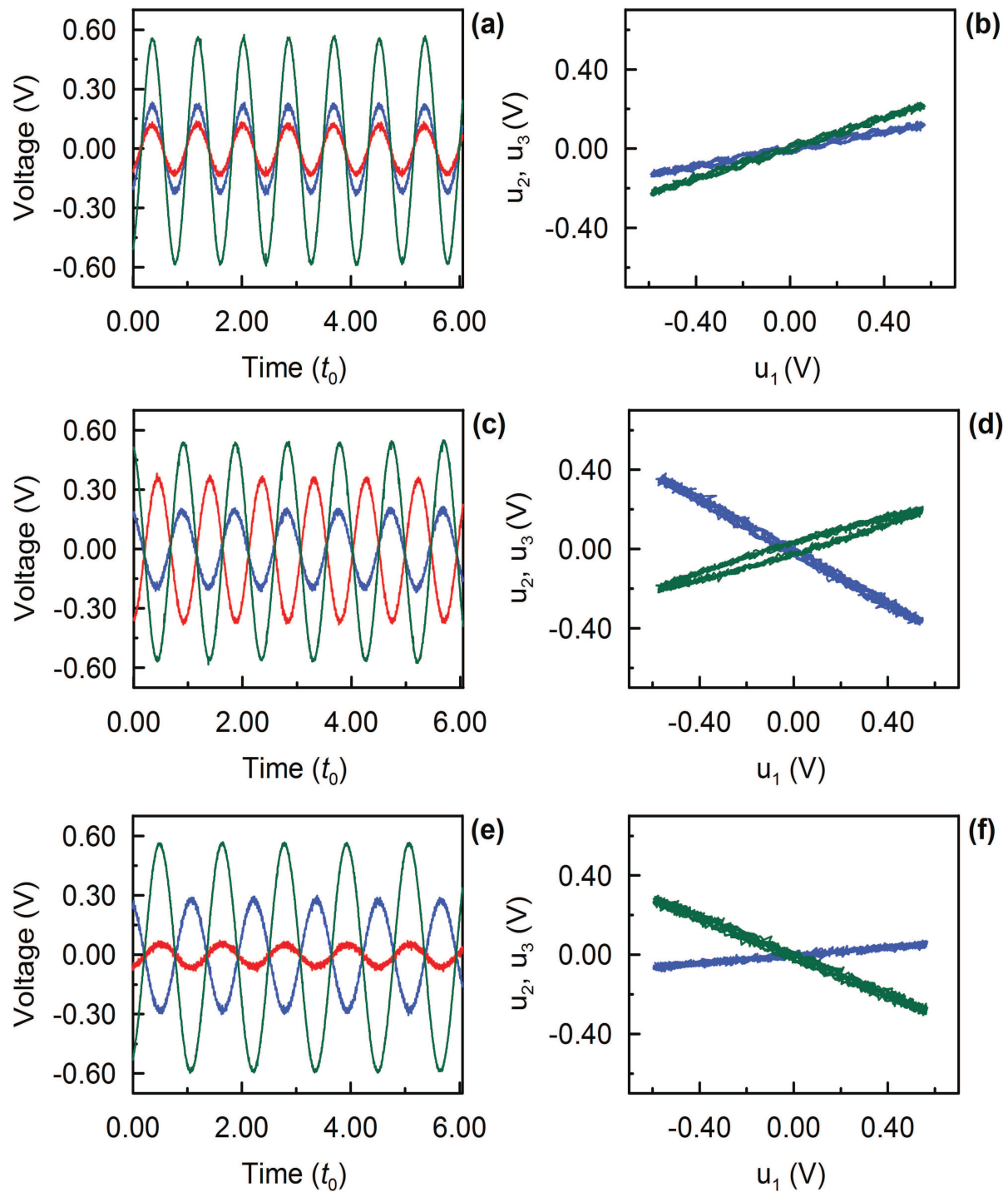
FIG. 7. Experimental time series and phase portraits of the system with one active (VDP) and two passive oscillators before [(a) and (b)], after the first (c) and (d), and after the second [(e) and (f)] bifurcation transition; C_4 = 150 pF [(a) and (b)], C_4 = 250 pF [(c) and (d)], and C_4 = 400 pF [(e) and (f)]. Green curve in the time series corresponds to the signal u_1 from the VDP oscillator (see Fig. 4), blue curve corresponds to the signal u_2 from the first passive oscillatory circuit, and red curve corresponds to the signal u_3 from the second passive oscillatory circuit.
