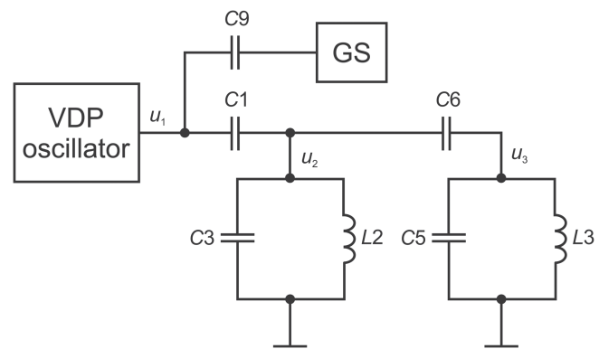
FIG. 8. The scheme of the CPG in the presence of noise or external forcing; C9 = C1 .
