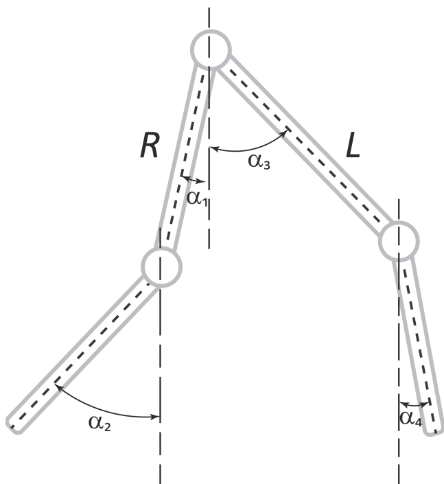
FIG. 11. Biped model with two joints per leg; “R” denotes the right leg and “L” denotes the left leg. All angles are measured positively clockwise from vertical.
