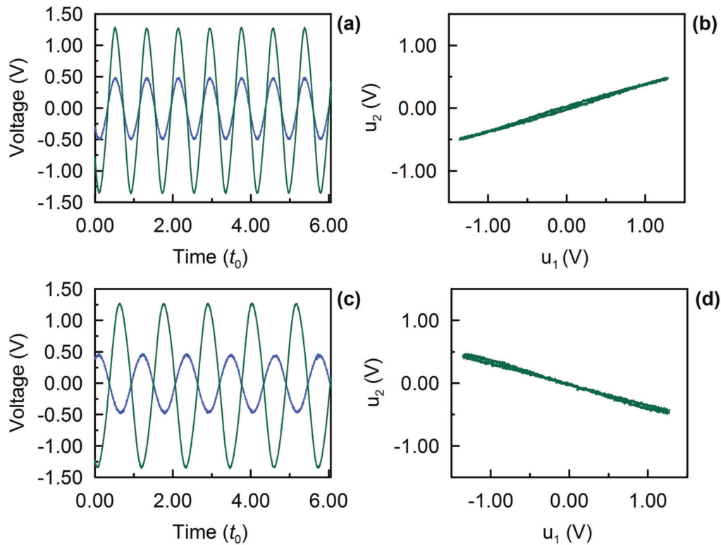
FIG. 3. Experimental time series [(a) and (c)] and corresponding phase portraits [(b) and (d)] of the system with one active (VDP) and one passive oscillators before [(a) and (b)] and after [(c) and (d)] the bifurcation transition; C_4 = 200 pF [(a) and (b)] and C_4 = 400 pF [(c) and (d)]. Green curve in time series corresponds to the signal u_1 from the VDP oscillator [see Fig. 1(a)] and blue curve corresponds to the signal u_2 from the passive oscillatory circuit.
