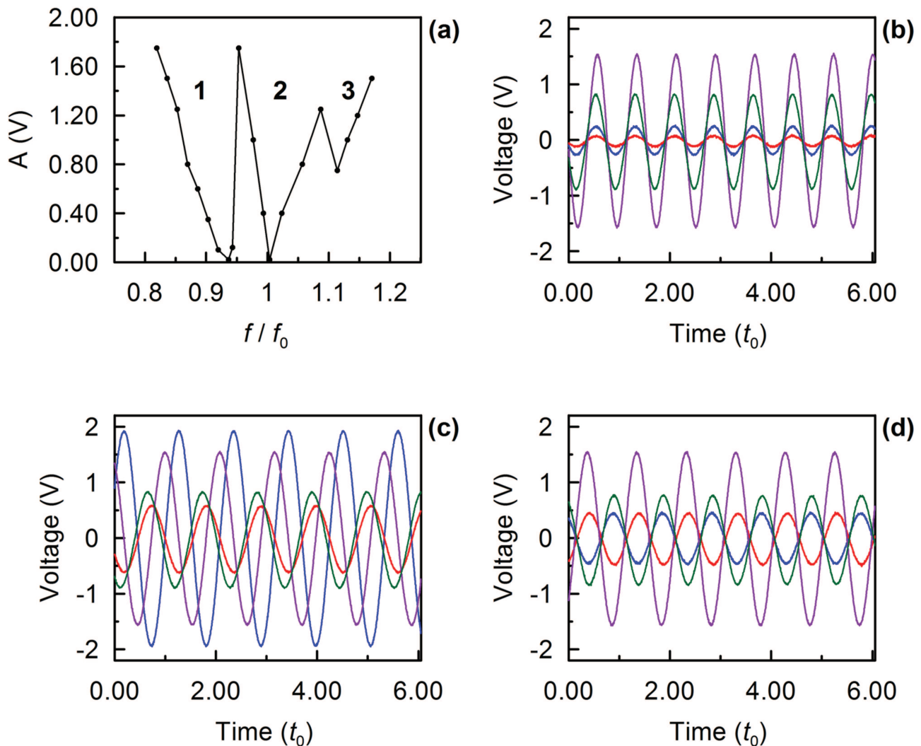
FIG. 10. (a) The chart of regimes of the CPG model under external harmonic forcing; C_4 = 170 pF. Experimental time series of the system for regime 3 ( f/f_0 = 1.13 ) on the chart (b), regime 1 ( f/f_0 = 0.93 ) (c), and regime 2 ( f/f_0 = 1 ) (d); A = 1.5 V. Green curve in the time series corresponds to the signal u_1 from the VDP oscillator (see Fig. 8), blue curve corresponds to the signal u_2 from the first passive oscillatory circuit, red curve corresponds to the signal u_3 from the second passive oscillatory circuit, and purple curve corresponds to the signal of the external harmonic forcing.
