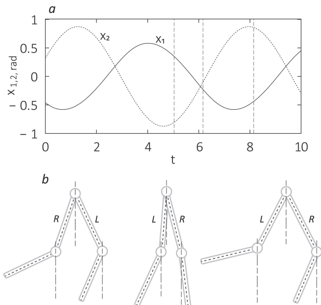
FIG. 12. (a) Time series generated by the CPG, which define the angular displacements for the thigh and shin of the first leg in the regime of running; x_1 is the signal from the VDP oscillator (see Fig. 4), x_2 is the signal from the first passive circuit; \tau = \pi , A = 0.03 , and f = 0.94 . (b) Snapshots of simulated biped running gait at the time moments denoted by vertical dashed lines in (a).
