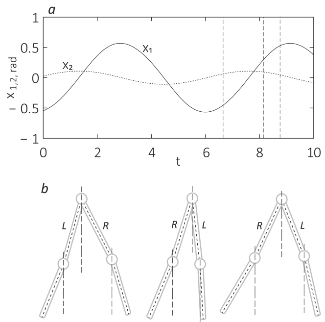
FIG. 14. (a) Time series generated by the CPG, which define the angular displacements for the thigh and shin of the first leg in the regime of walking; \tau = \pi and A = 0 . (b) Snapshots of simulated biped walking gait at the time moments denoted by vertical dashed lines in (a).
