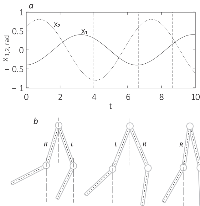
FIG. 13. (a) Time series generated by the CPG, which define the angular displacements for the thigh and shin of the first leg in the regime of running that is slower than running regime in Fig. 12; \tau = \pi , A = 0.03 , and f = 0.943 . (b) Snapshots of simulated biped slow running gait at the time moments denoted by vertical dashed lines in (a).
