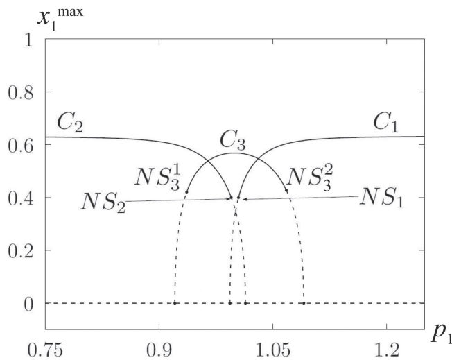
FIG. 5. Characteristic bifurcation diagram for the model (7) with two passive coupled oscillators. Here, C_{1,2,3} are the limit cycles, NS_{1,2} and NS_3^{1,2} are the bifurcation points for Neimark–Sacker bifurcation. The dashed lines represent unstable limit sets, while the solid lines represent stable limit cycles.
