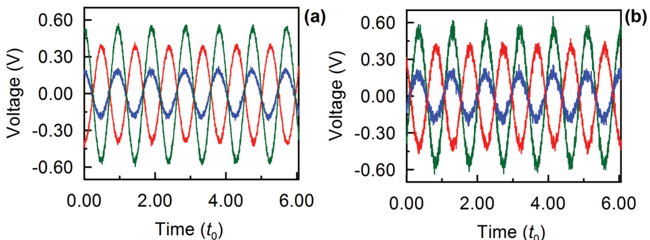
FIG. 9. Experimental time series of the system with one active and two passive oscillators ( C4 = 250 pF) for the following values of the external noise intensities: (a) SNR = 24 dB and (b) SNR = 12 dB. Green curve in the time series corresponds to the signal u_1 from the VDP oscillator (see Fig. 8), blue curve corresponds to the signal u_2 from the first passive oscillatory circuit, and red curve corresponds to the signal u_3 from the second passive oscillatory circuit.
