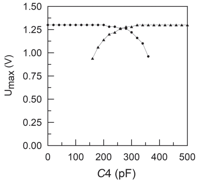
FIG. 2. The amplitude of voltage oscillations in the active self-sustained oscillator of the coupled system (see Fig. 1) vs the value of C_4 capacitance.
