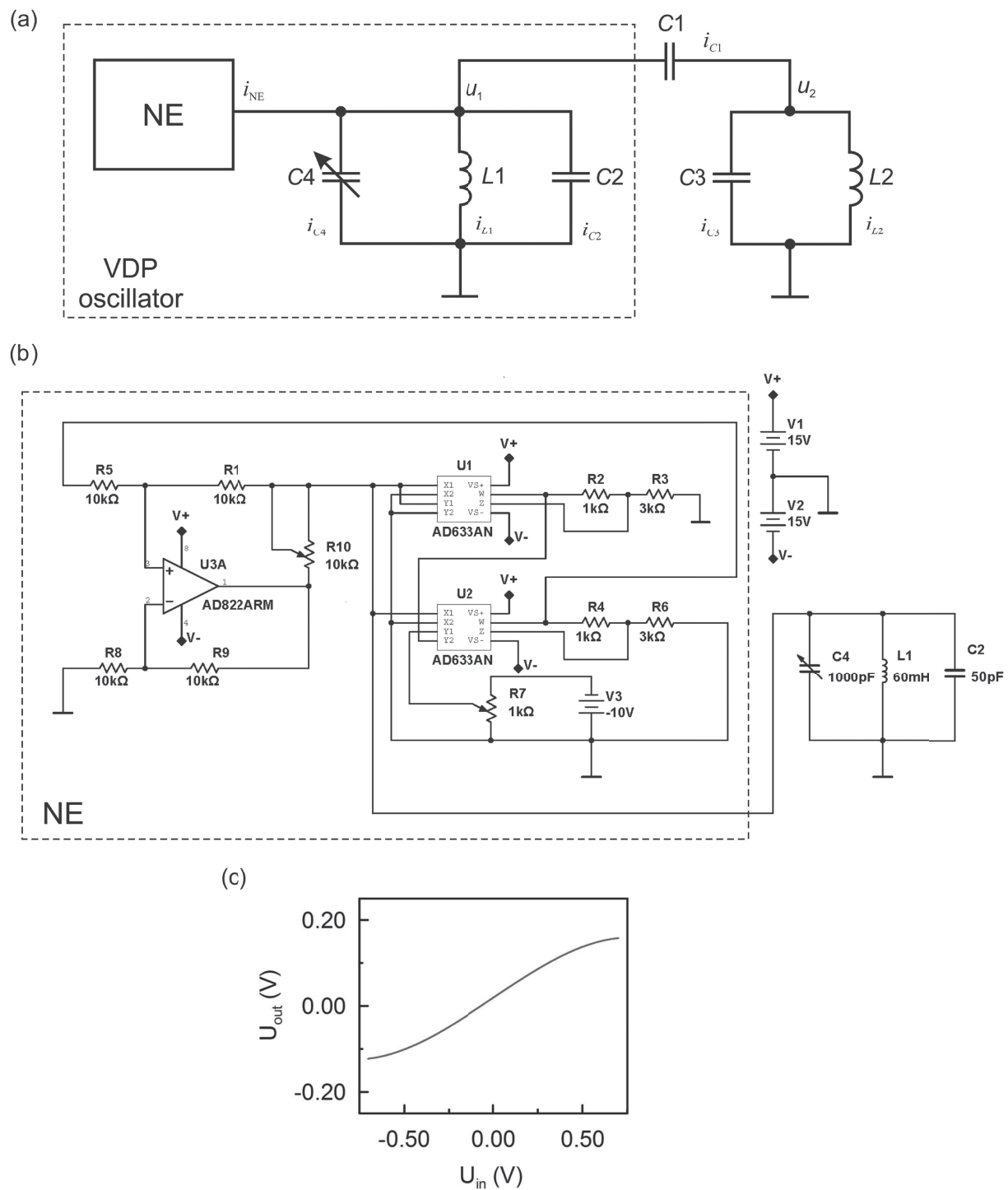
FIG. 1. The scheme of the CPG based on the active VDP oscillator coupled to the passive oscillatory circuit: (a) the general scheme, where "NE" denotes a nonlinear element of Van der Pol oscillator; (b) detailed electronic scheme of the implemented Van der Pol oscillator; (c) the transfer characteristic of the nonlinear element, which is well described by a cubic polynomial function.
