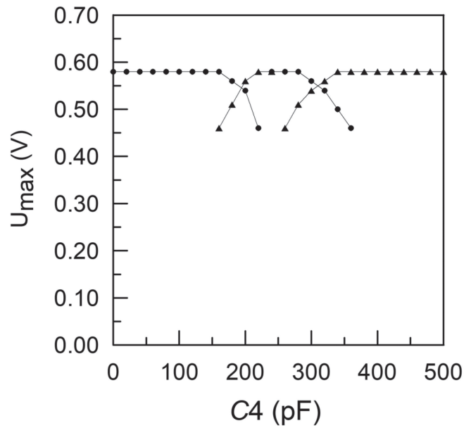
FIG. 6. The amplitude of voltage oscillations in the active oscillator of the system (see Fig. 4) vs the value of C_4 capacitance.
