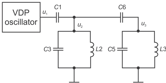
FIG. 4. The scheme of the CPG based on the active VDP oscillator coupled with two passive oscillators. Here, C_5 = C_3 , L_3 = L_2 , and C_6 = C_1 .
